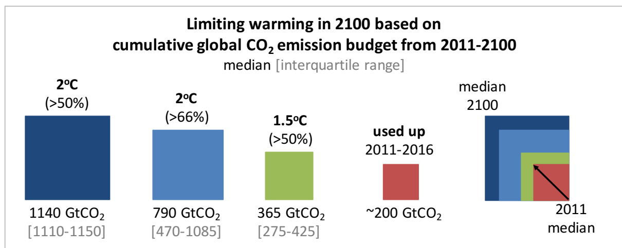
FIGURE 1. CUMULATIVE EMISSION BUDGETS FOR LIMITING WARMING TO 2°C AND 1.5°C. NOTES: AREAS OF BOXES ARE PROPORTIONAL TO CUMULATIVE TOTAL CO 2 EMISSION BUDGETS FROM 2011 TO 2100 CONSISTENT WITH LIMITING WARMING TO 2°C AND 1.5°C (WITH 50–66% AND >66% PROBABILITY) BASED ON DATA FROM ROGELJ ET AL. (2015). HISTORICAL ANNUAL EMISSIONS OF ~40 GtCO 2 FROM 2011 TO 2016 ARE ESTIMATED FROM GCP (2016). NOTE THAT CUMULATIVE EMISSION BUDGETS VARY DEPENDING ON THE METHODOLOGY AND ASSUMPTIONS (ROGELJ ET AL., 2016). BUDGETS FOR LIMITING WARMING TO 2°C GIVEN IN THE IPCC FIFTH ASSESSMENT REPORT (CLARKE ET AL., 2014) ARE SLIGHTLY HIGHER AT 960–1430 GtCO 2 (50–66% PROBABILITY) AND 630–1180 GtCO 2 (>66% PROBABILITY). BUDGETS FOR LIMITING WARMING TO 1.5°C, REPORTED IN ROGELJ ET AL. (2015) ARE SLIGHTLY LOWER AT 200–415 GtCO 2 (>50% PROBABILITY).
